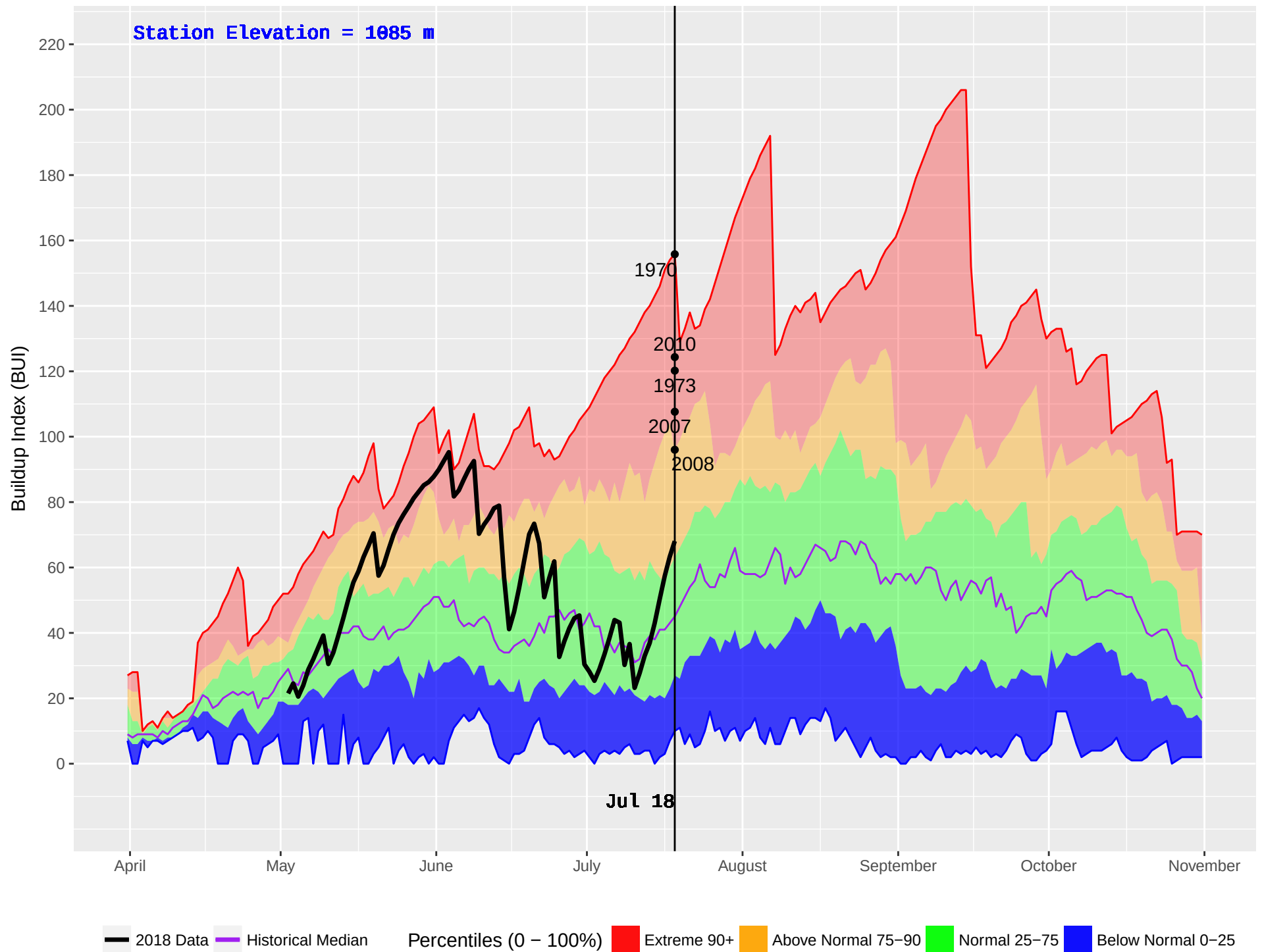
TAUTRI (206) : Historical (1970–2016) and Current (2018) Daily Buildup Index (BUI)
