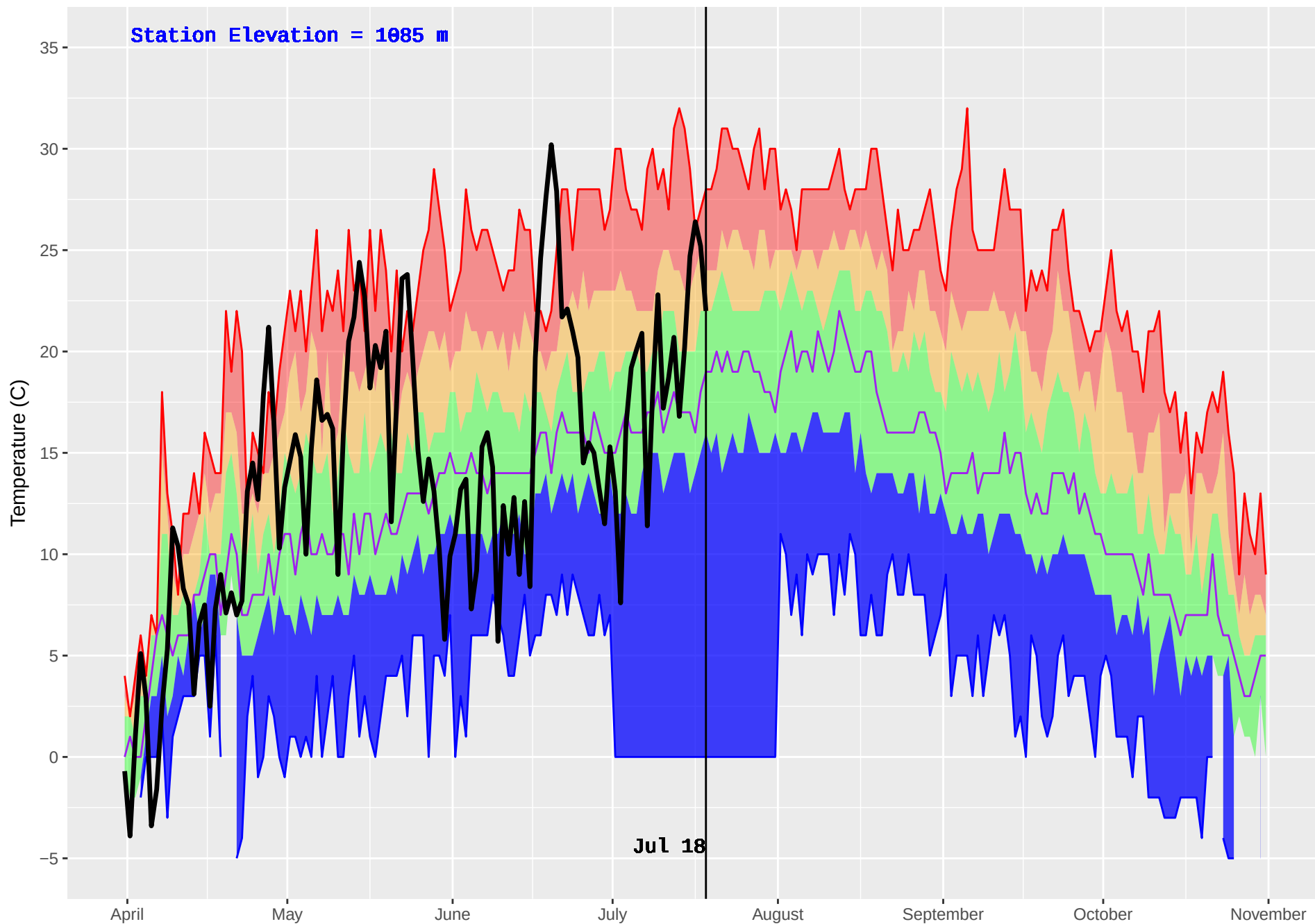
TAUTRI (206) : Historical (1970–2016) and Current (2018) Daily Temperature
