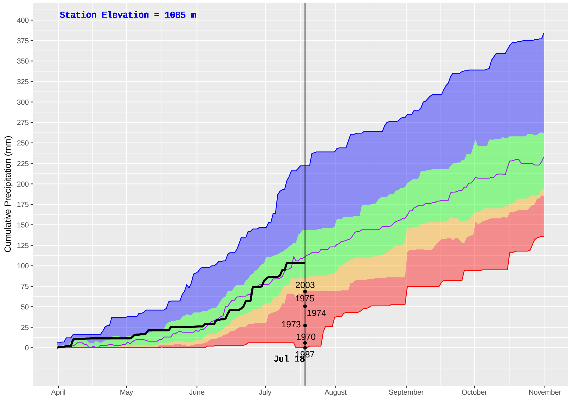
TAUTRI (206) : Historical (1970–2016) and Current (2018) Daily Cumulative Precipitation
