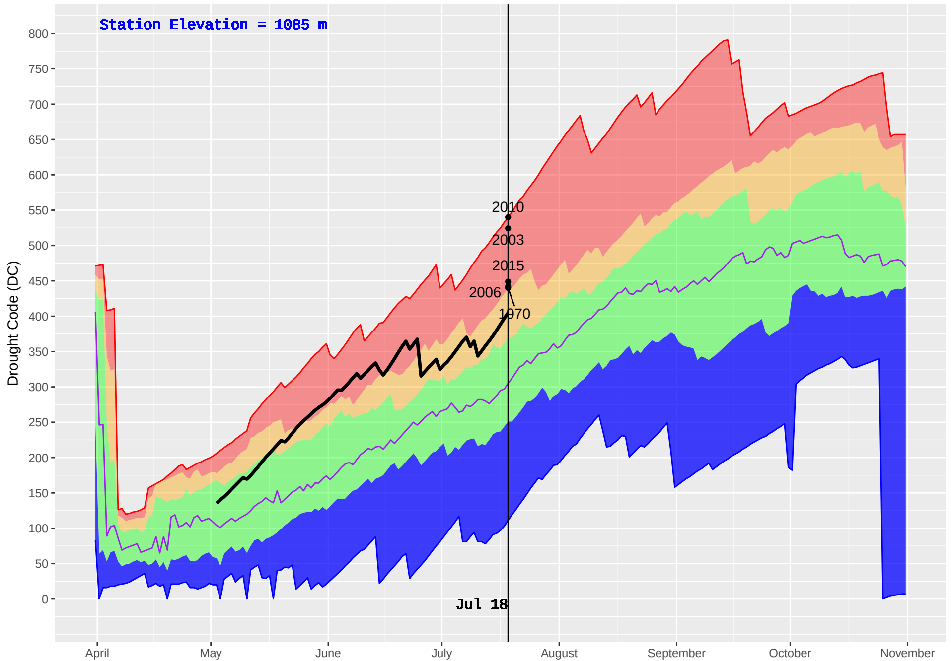
TAUTRI (206) : Historical (1970–2016) and Current (2018) Daily Drought Code (DC)
