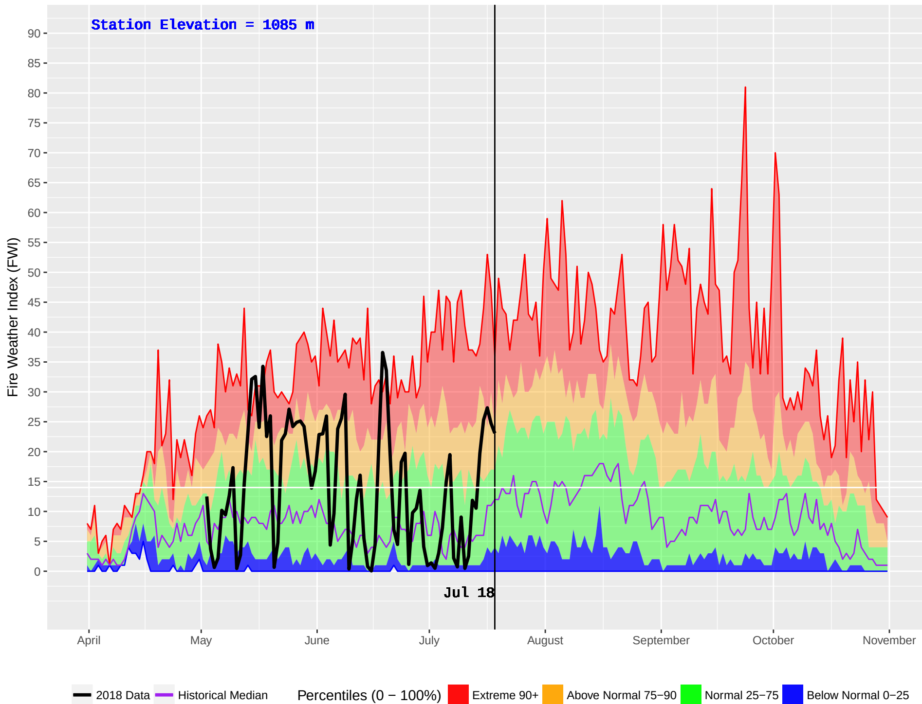
TAUTRI (206) : Historical (1970–2016) and Current (2018) Daily Fire Weather Index (FWI)
