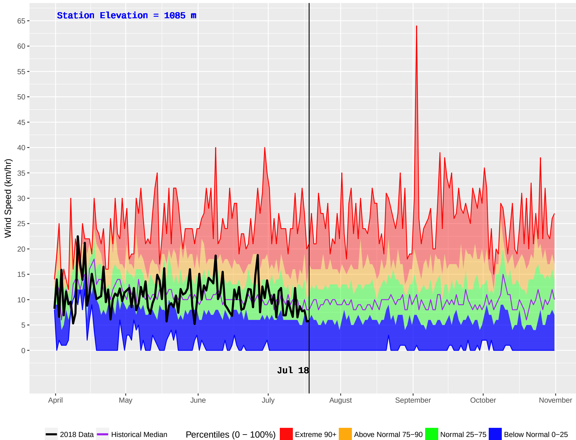
TAUTRI (206) : Historical (1970–2016) and Current (2018) Daily Wind Speed
