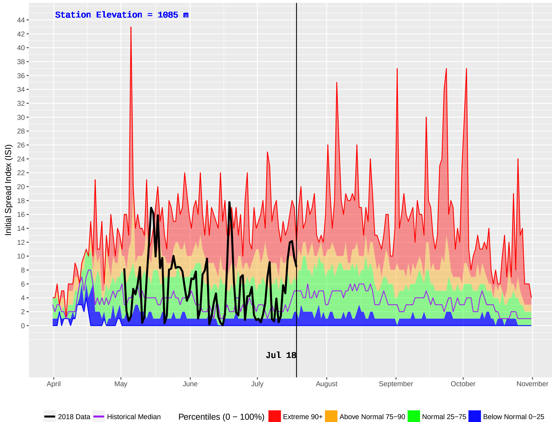
TAUTRI (206) : Historical (1970–2016) and Current (2018) Daily Initial Spread Index (ISI)
