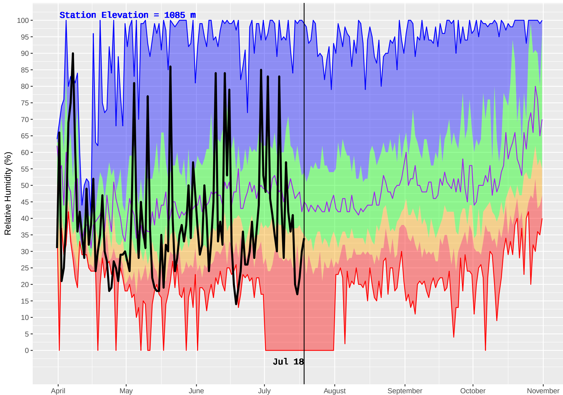
TAUTRI (206) : Historical (1970–2016) and Current (2018) Daily Relative Humidity
